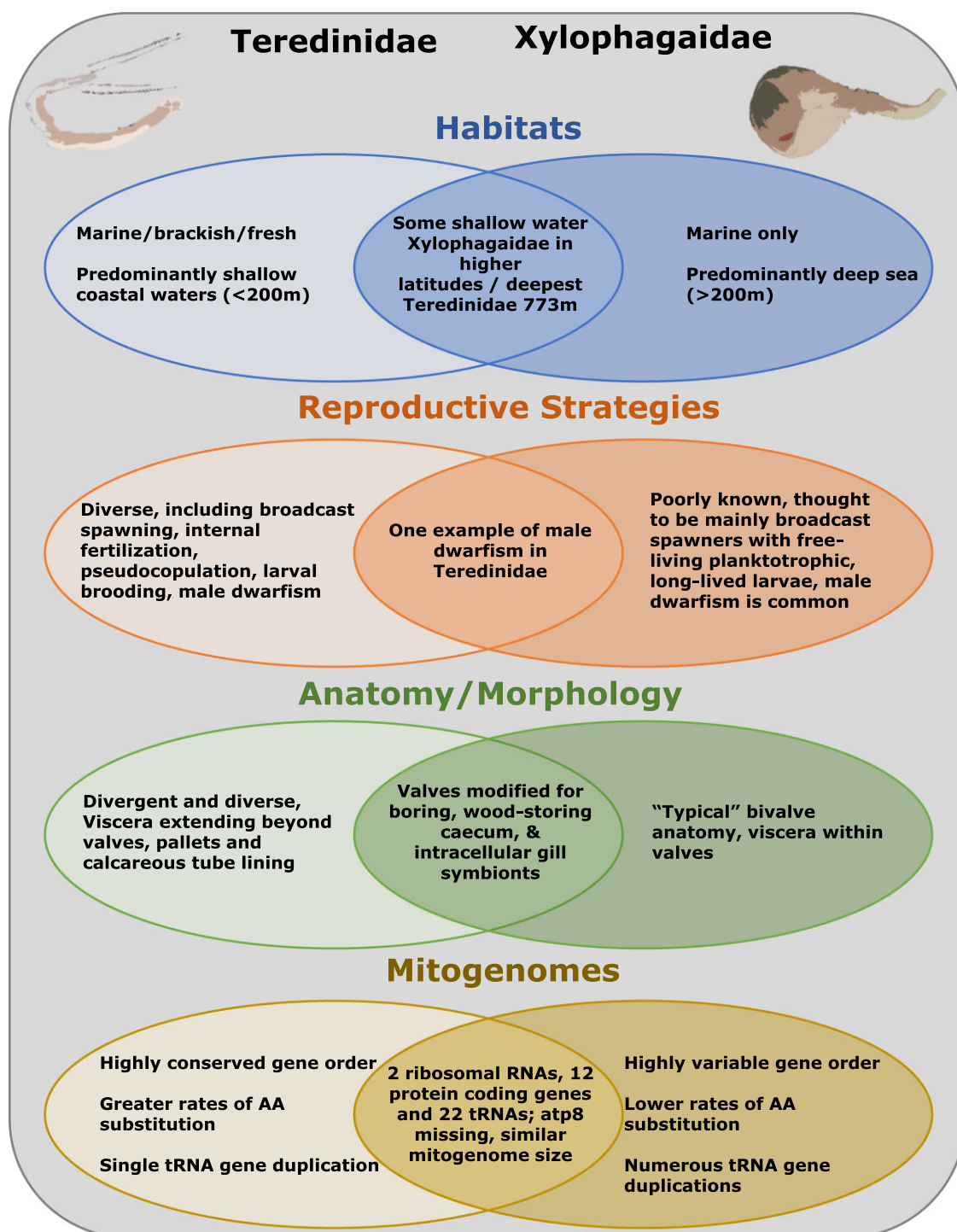
FIG. 2. —Graphic comparison of teredinid and xylophagaid habitat preferences, reproductive strategies, anatomy, and mitochondrial genome characteristics.
